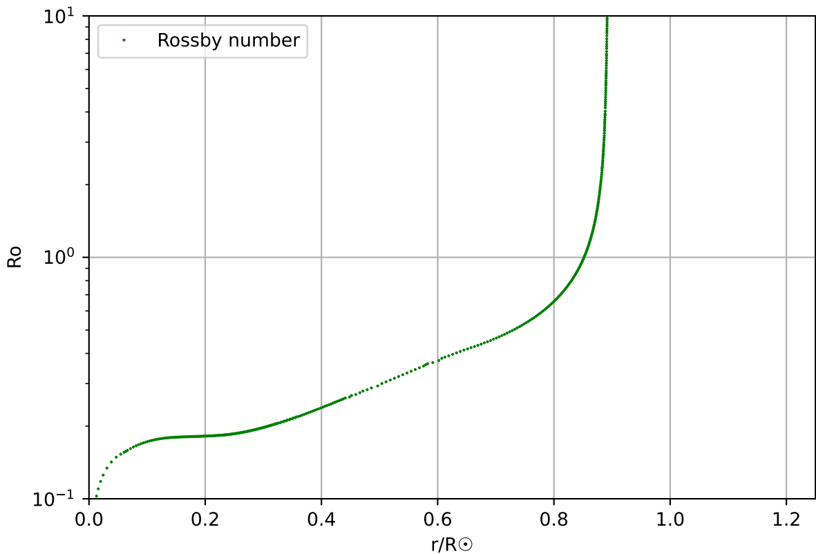
Rossby number, profile 128, age 1.94 \times 10^8
